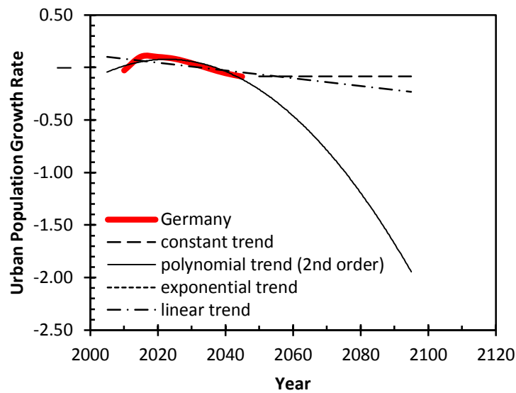
Predicted urban growth for large urban areas in Germany
